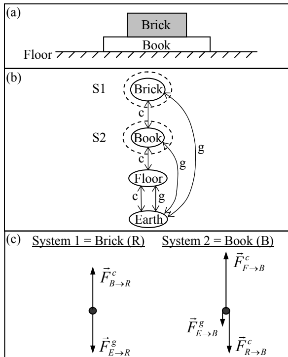
FIGURE 1. (a) Pictorial representation of a physical situation. All objects are at rest. (b) System schema of this physical situation, with two of many possible systems identified. The dashed ellipses represent system 1 (S1) and system 2 (S2) respectively. “c” labels a contact interaction, and “g” labels a gravitational interaction. (c) Free-body diagrams for the two systems identified in (b). In a force label “c” means contact, “g” means gravitational. Also, for this particular scenario “B” means book, “R” means brick, “E” means earth, and “F” means floor. For example, the symbol \vec{F}_{B \rightarrow R}^c means a contact force by the book on the brick. Note the mass of the brick has arbitrarily been chosen to be three times the mass of the book, thus \vec{F}_{E \rightarrow R}^g is three times the length of \vec{F}_{E \rightarrow B}^g .
